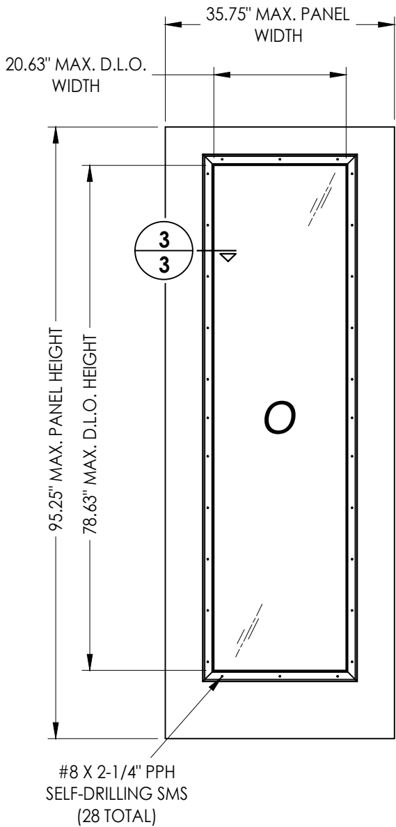
51 FIBERGLASS SIDELITE PANEL ODL w/ KEYSTONE PVC LITE FRAME
