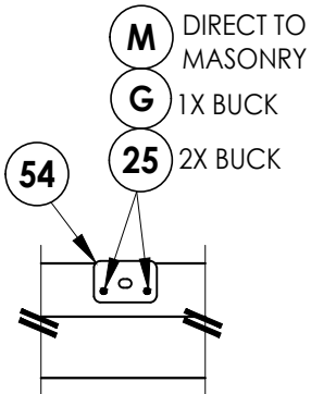
ASTRAGAL BOLT DETAIL STRIKE PLATE @ HEAD
