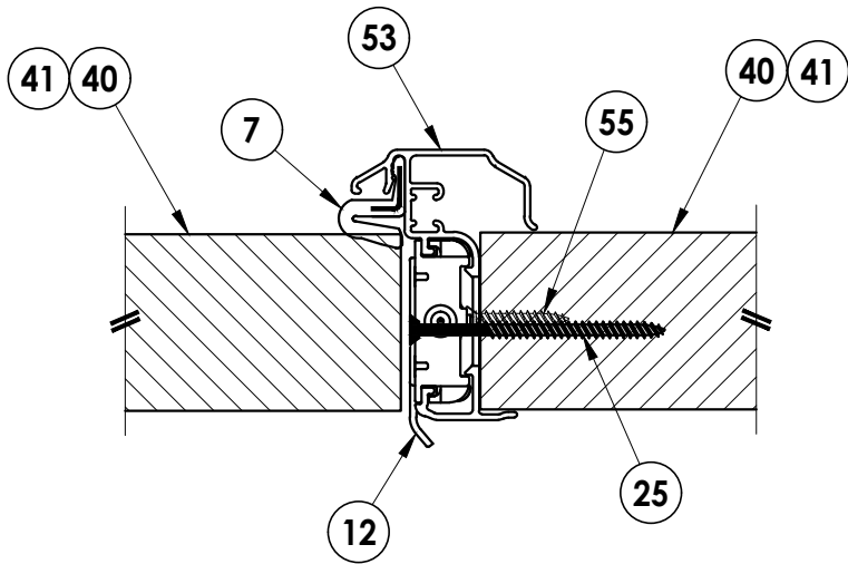
1 7 HORIZONTAL CROSS SECTION Outswing Shown (Inswing Similar)
