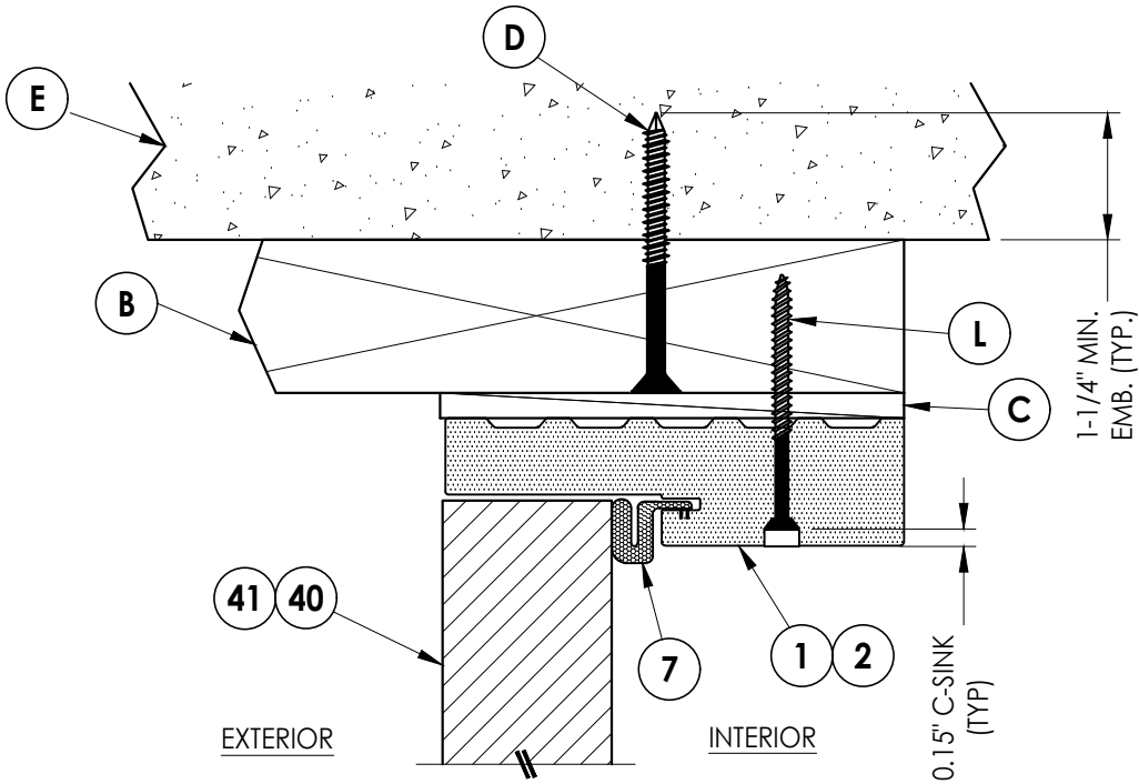
3 8 VERTICAL CROSS SECTION Outswing Shown (Inswing Similar) Shown w/ 2X Buck
