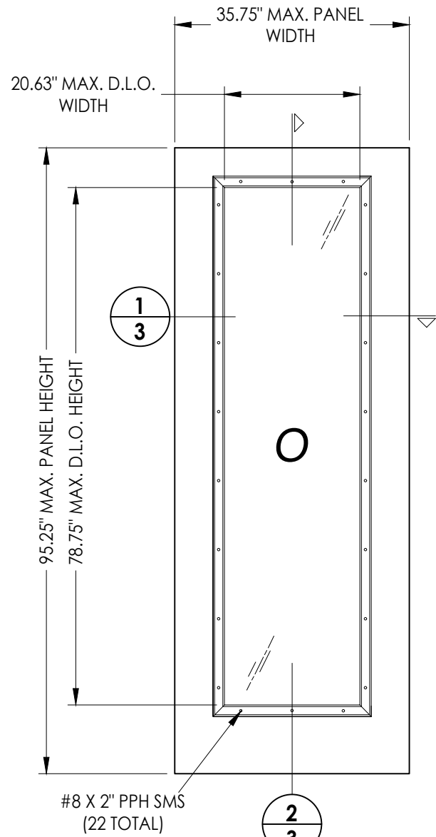
50 FIBERGLASS SIDELITE PANEL ODL w/ FLAT ALUM. LITE FRAME
